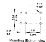
Mounting (Bottom view)
