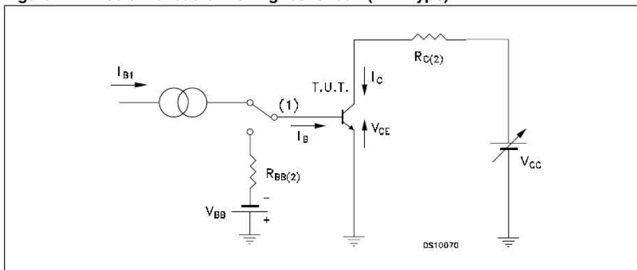
Figure 2. Resistive load switching test circuit (NPN type)
