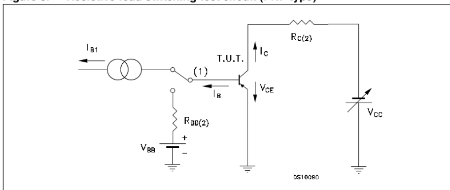
Figure 3. Resistive load switching test circuit (PNP type)
