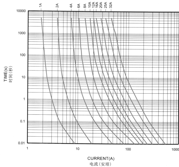
HC10gG AVERAGE I-T CHARACTERISTICS CURVE (FOR REFERENCE)
