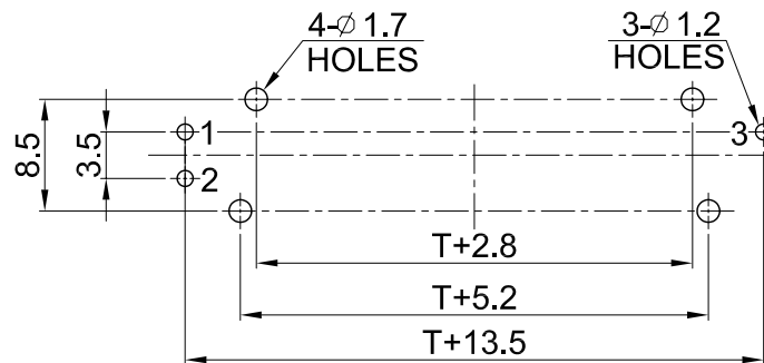
P. C. B MOUNTING DETAIL
