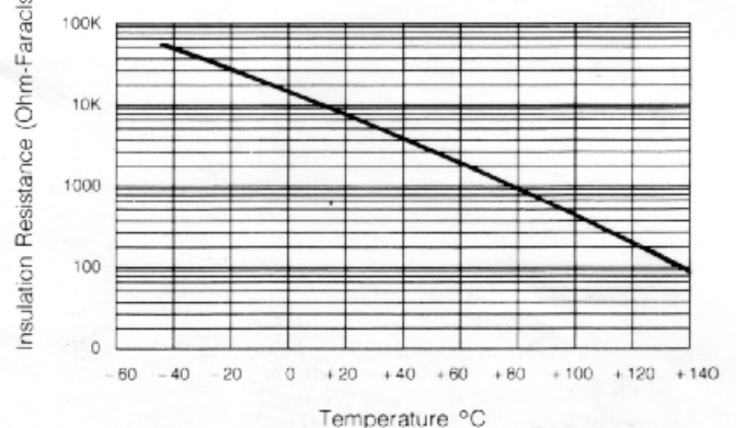
Insulation Resistance VS. Temp.
