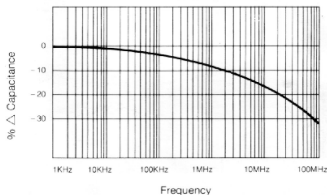
\Delta C , VS. Frequency Coefficient
