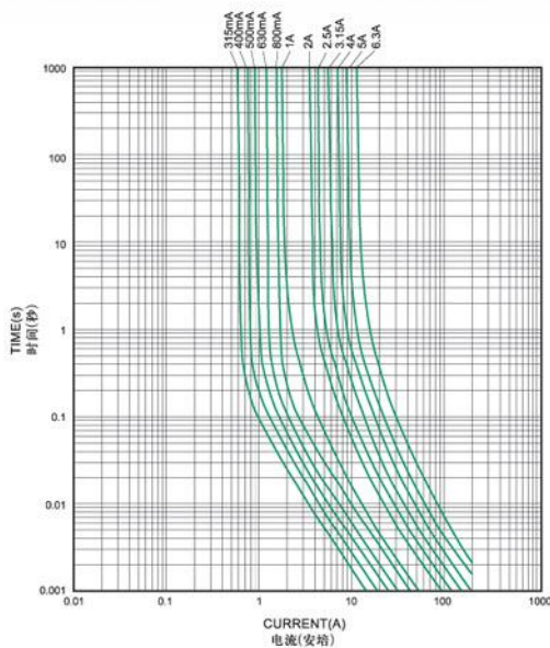
5RF RoHS I-T CHARACTERISTICS CURVE 5RF RoHS 电流-时间曲线图
