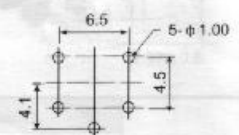
P.C.B. HOLE DETAIL
