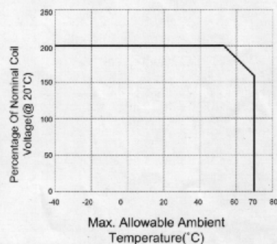
MAX.ALLOWABLE AMBIENT TEMPERATURE CURVE
