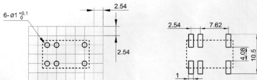
PCB layout
