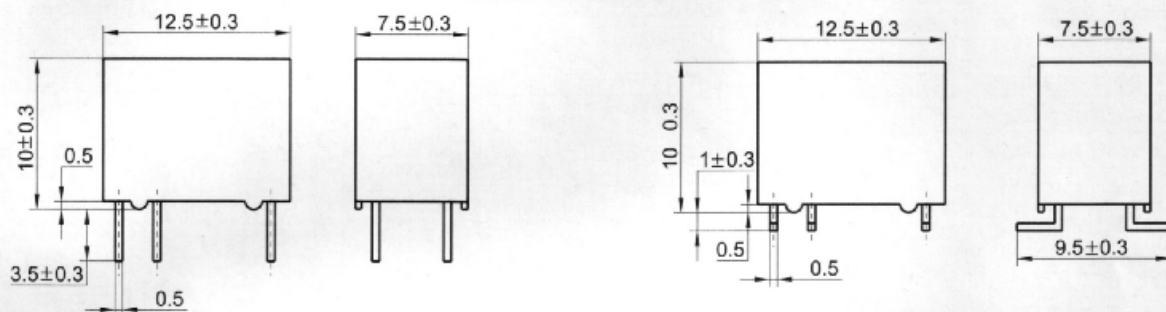
Outline Dimensions
