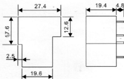
SEALED TYPE
