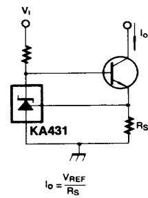
Figure 15. Constant-Current Sink
