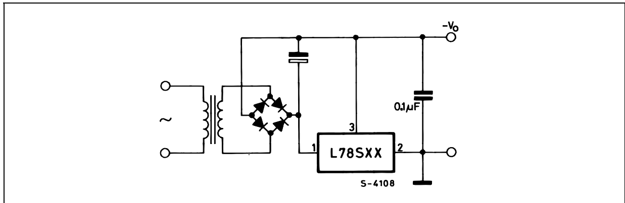
Figure 23 : Switching Regulator
